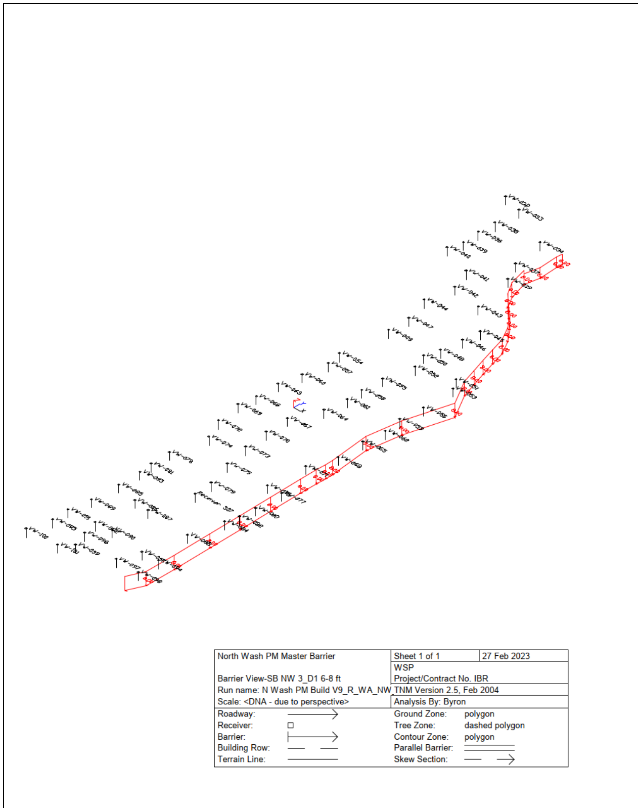
Figure L-3. TNM Noise Wall Graphic – Noise Wall 3
