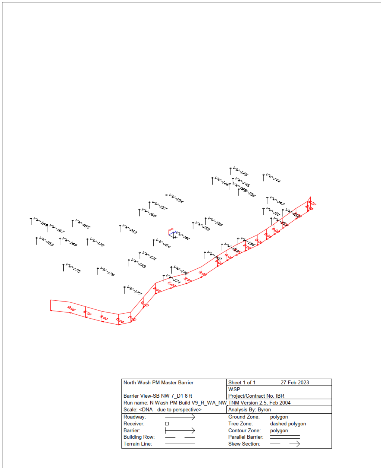
Figure L-7. TNM Noise Wall Graphic – Noise Wall 7
