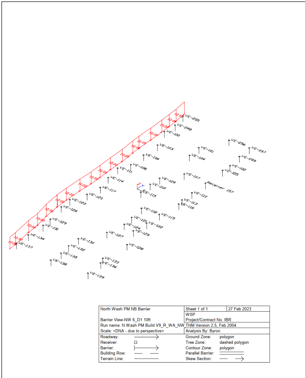
Figure L-6. TNM Noise Wall Graphic – Noise Wall 6
